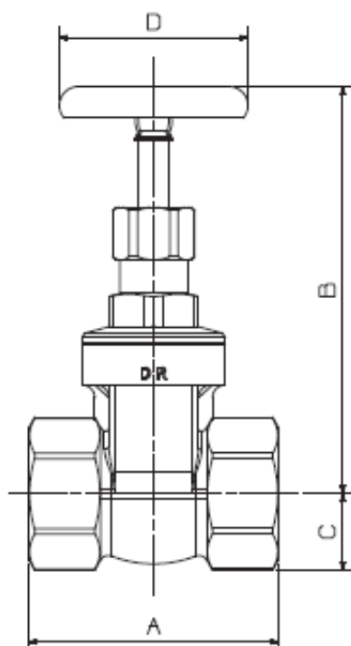
Figure 2: LINE DRAWING
