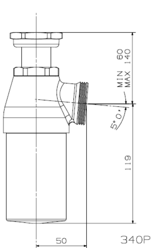
Figure 2: LINE DRAWING
