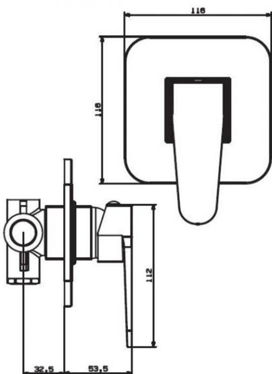
Figure 2: LINE DRAWING
