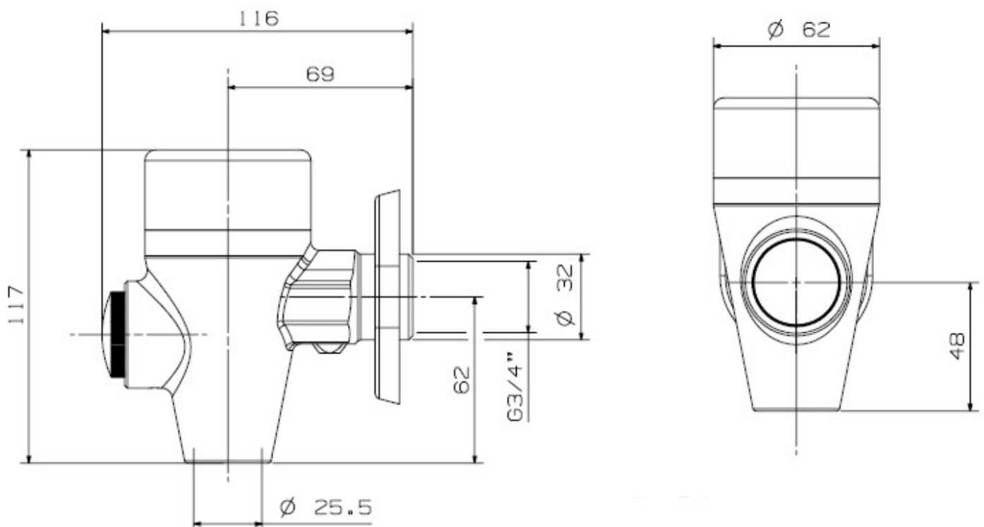
Figure 2: LINE DRAWING
