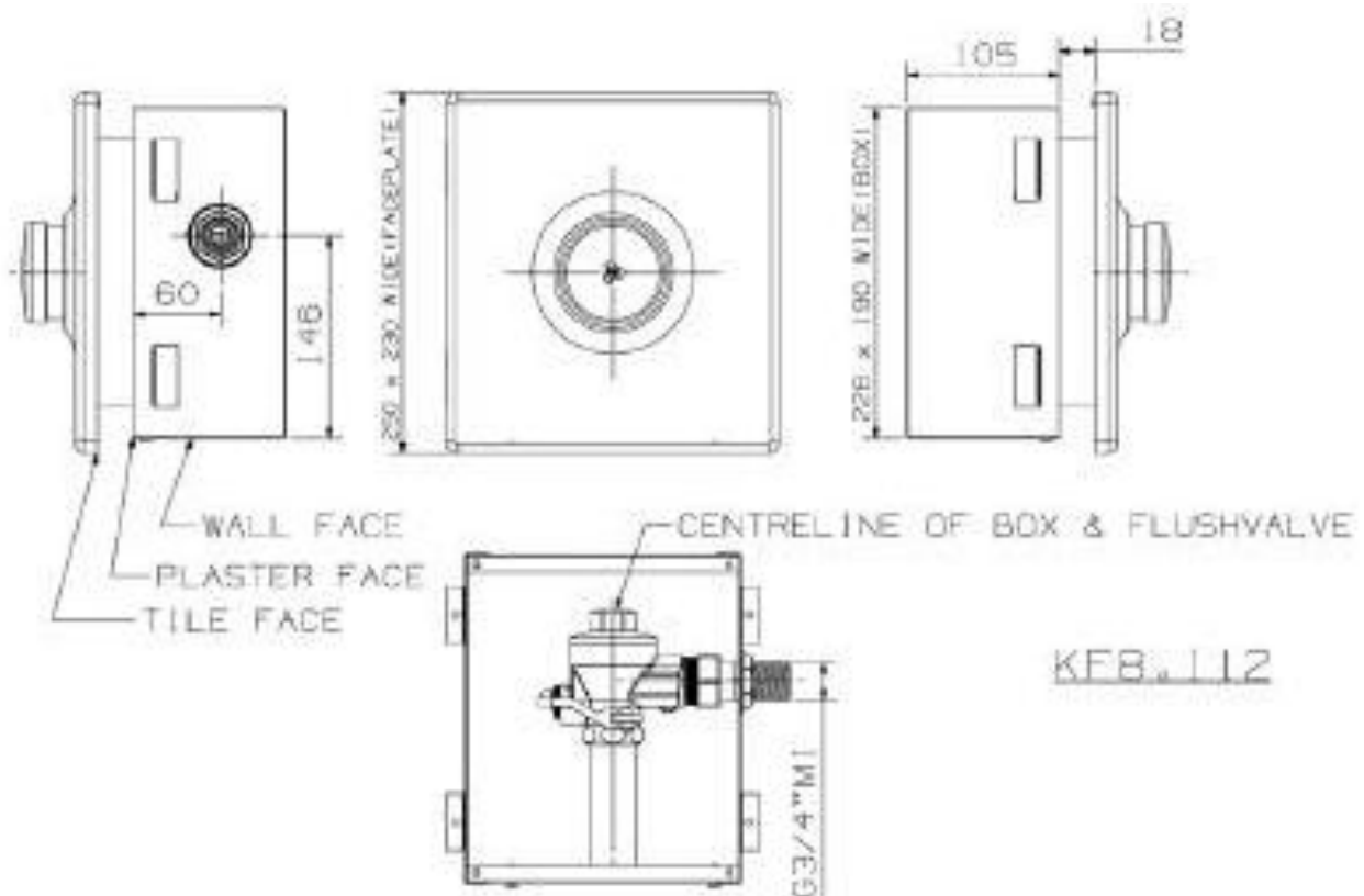
Figure 2: LINE DRAWING
