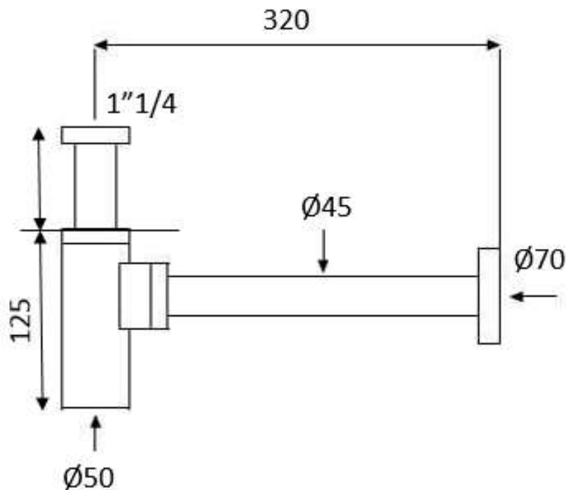
Figure 2: LINE DRAWING
