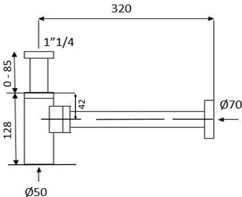
Figure 2: LINE DRAWING
