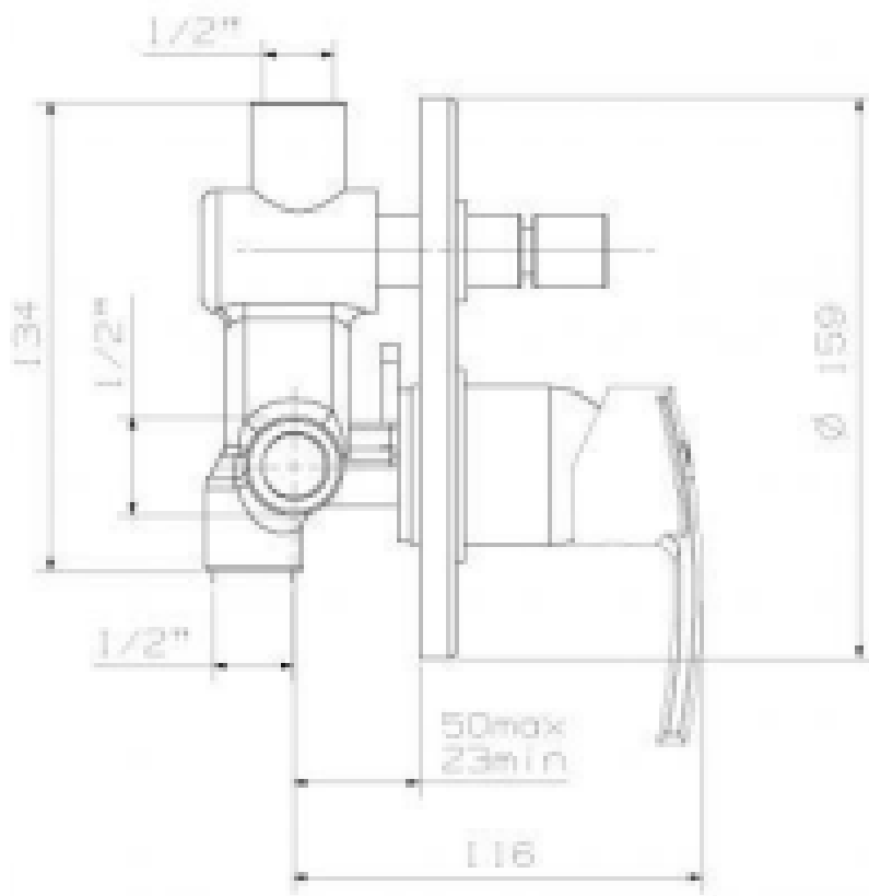
Figure 2: LINE DRAWING
