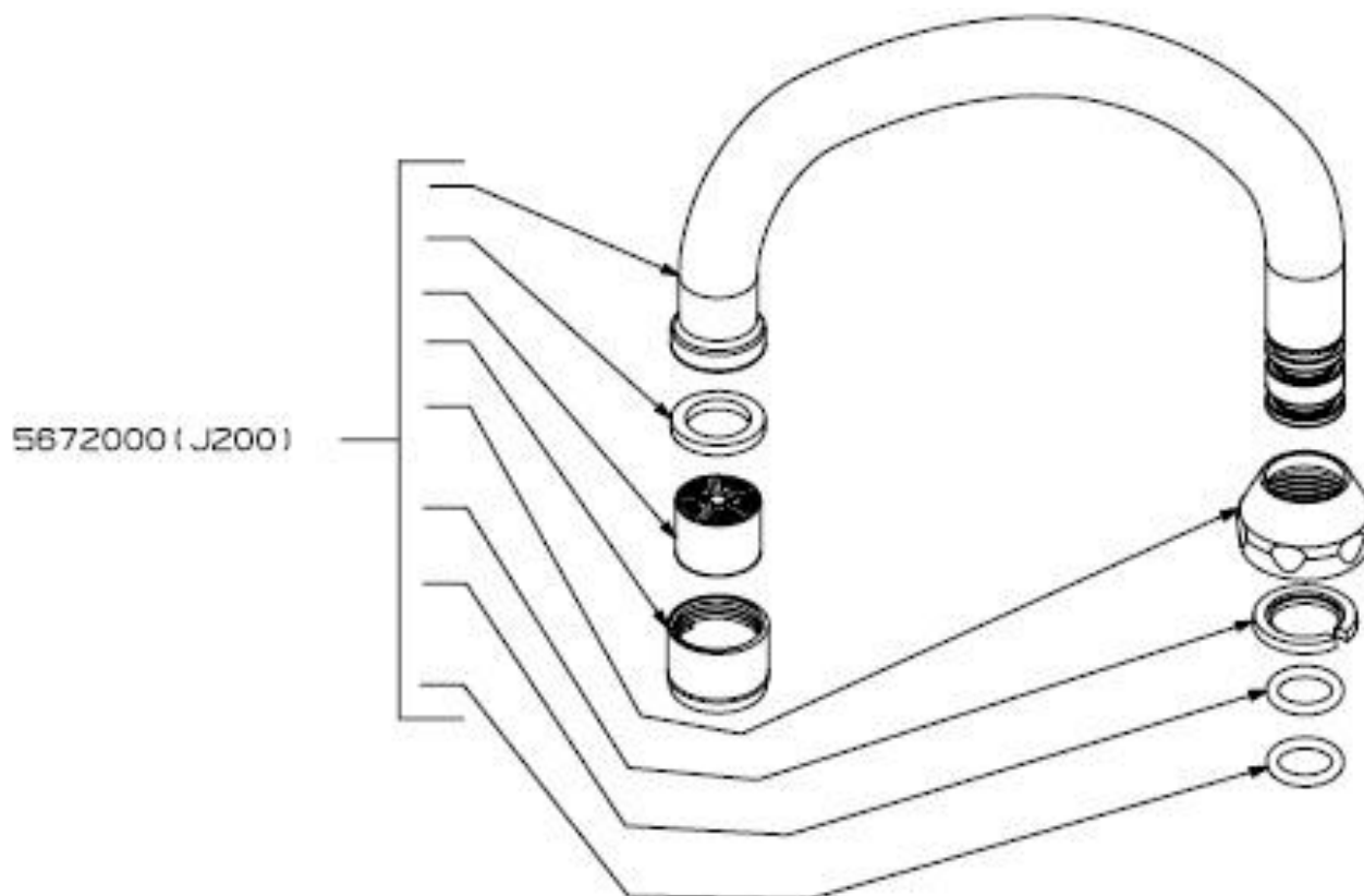
Figure 2: LINE DRAWING
