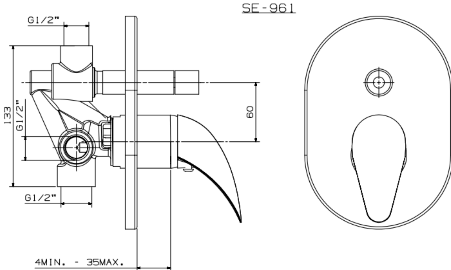
Figure 2: LINE DRAWING
