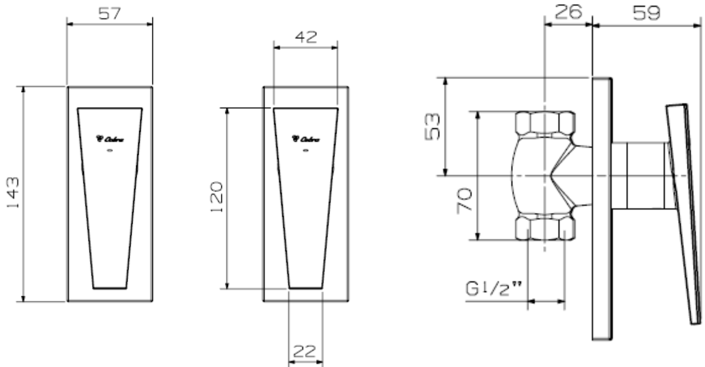
Figure 2: LINE DRAWING
