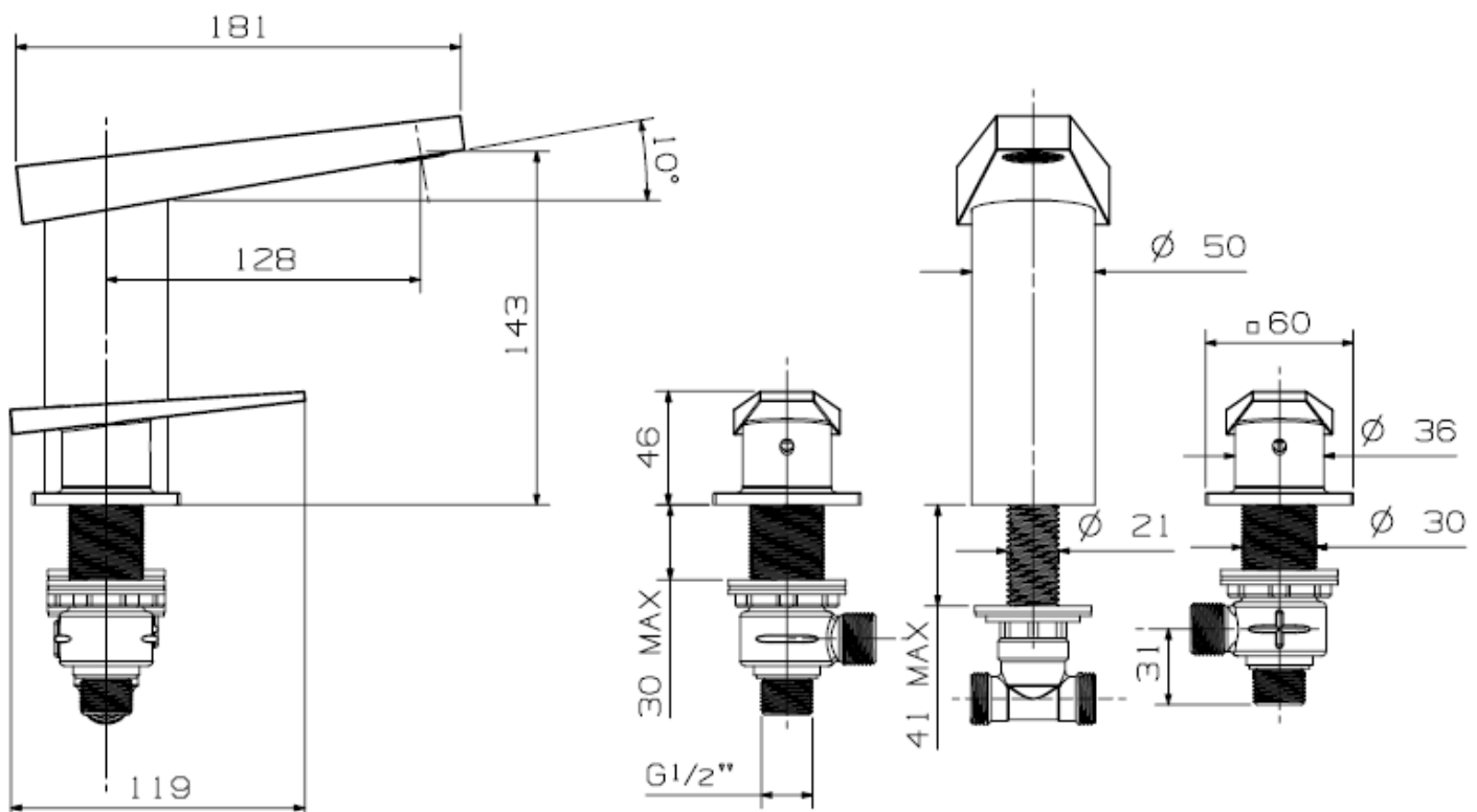
Figure 2: LINE DRAWING
