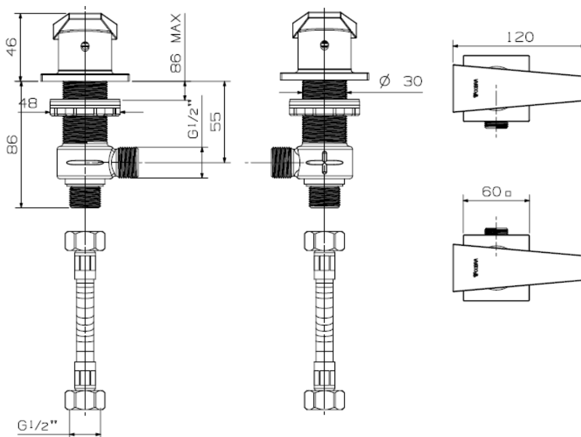
Figure 2: LINE DRAWING
