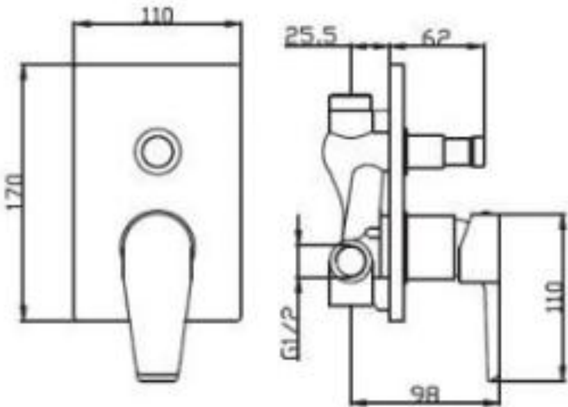
Figure 2: LINE DRAWING
