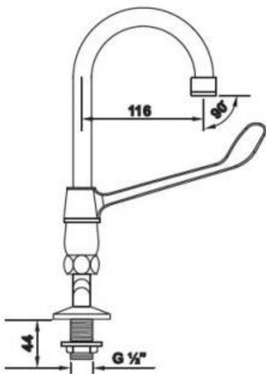
Figure 2: LINE DRAWING
