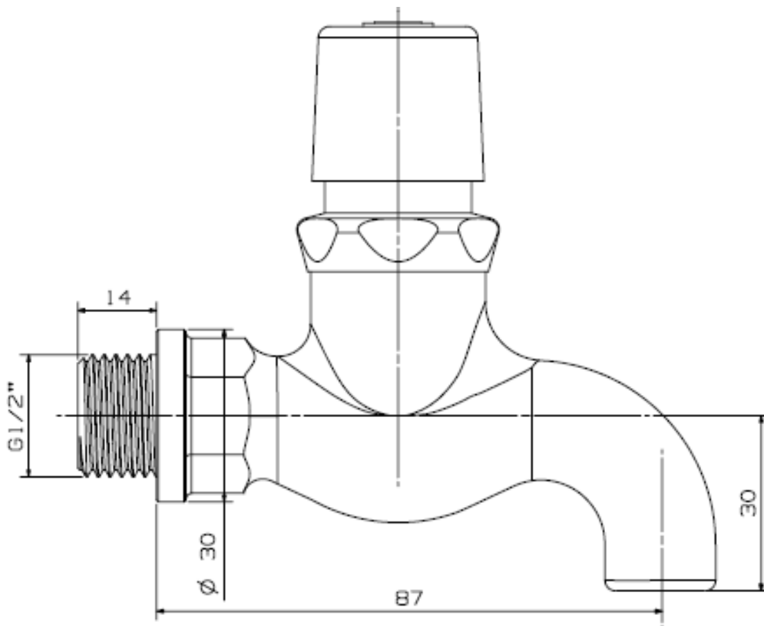
Figure 2: LINE DRAWING
